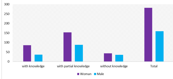
Frequency Distribution
